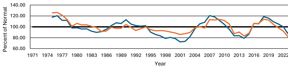
5-Year Moving Average of Percent of Normal Rainfall Inside (blue) vs. East (Orange) of the WTWMA Target Area
